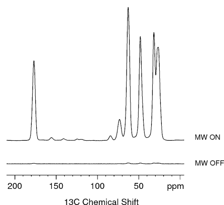
Figure 1. ^{13}\text{C} CPMAS spectra of 0.25 M U- ^{13}\text{C} - ^{15}\text{N} proline with 10 mM AMUPol in [D 8 ]glycerol/D 2 O/H 2 O (60/30/10 volume ratio) with (top trace) and without (bottom trace) microwave irradiation at 14 kHz MAS, 97 K sample temperature, 8 scans, 1 dummy scan, 6.4 s recycle delay, 9 W microwave power at end of probe waveguide.
